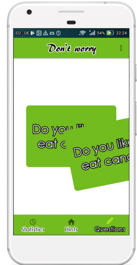
Swipecards library
