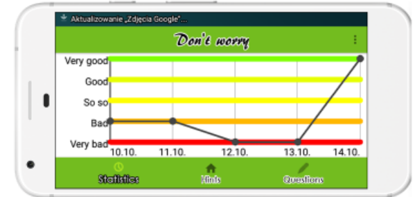
Graph View Library
